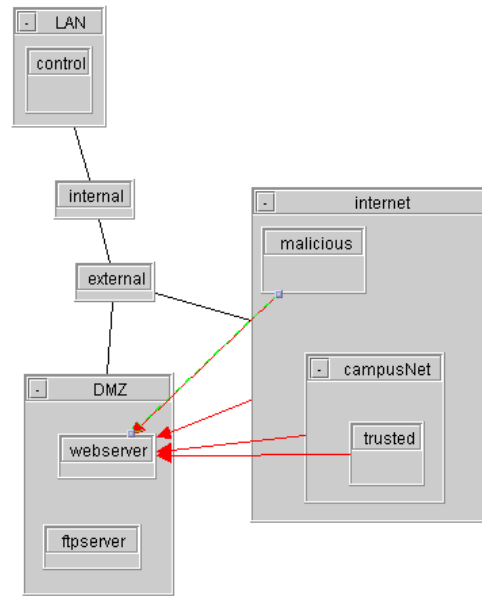
Figure 6. Picture of overlap mistake
